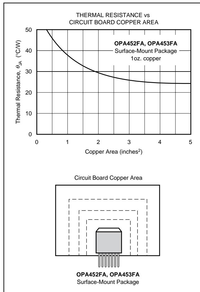
FIGURE 4. DDPAK Thermal Resistance vs Circuit Board Copper Area.
