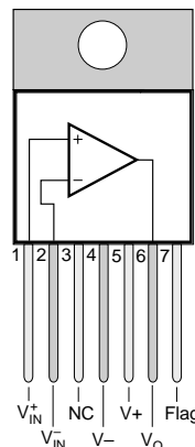
7-Lead Straight-Formed TO-220 (TA)
