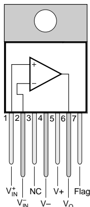
7-Lead Stagger-Formed TO-220 (TA-1)
