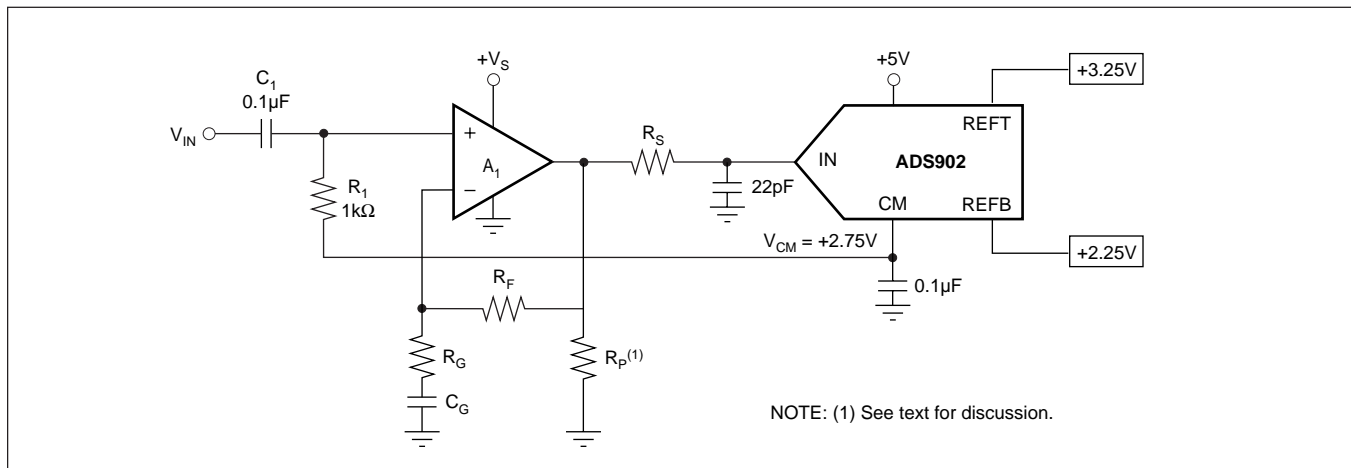
FIGURE 4. AC-Coupled, Single-Supply Interface Circuit.
